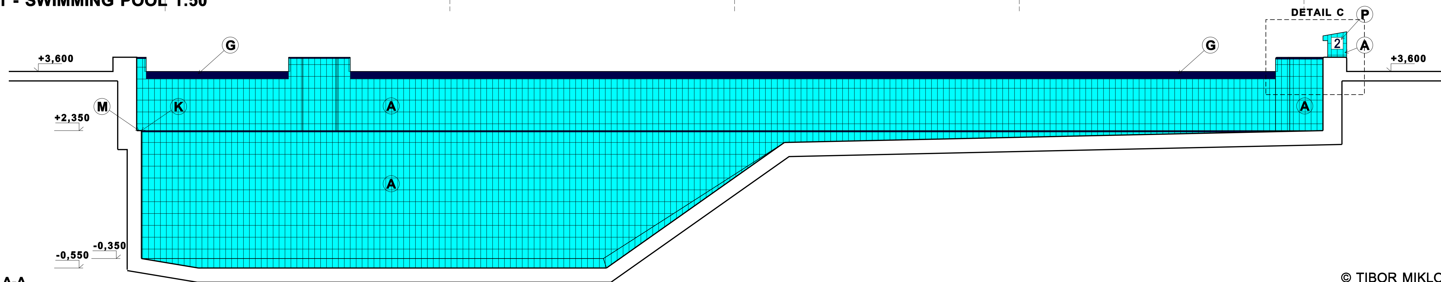
LEVEL 1 - SWIMMING POOL 1:50
